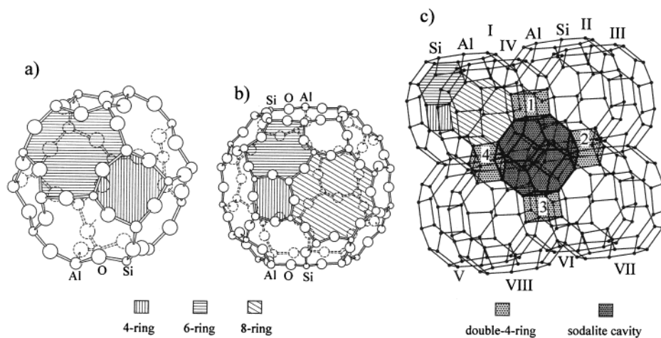
Figure 1. Representation of the structure of zeolite A: (a) \beta -cage (or sodalite cage), (b) \alpha -cage, (c) unit structure cell (oxygen not shown),
